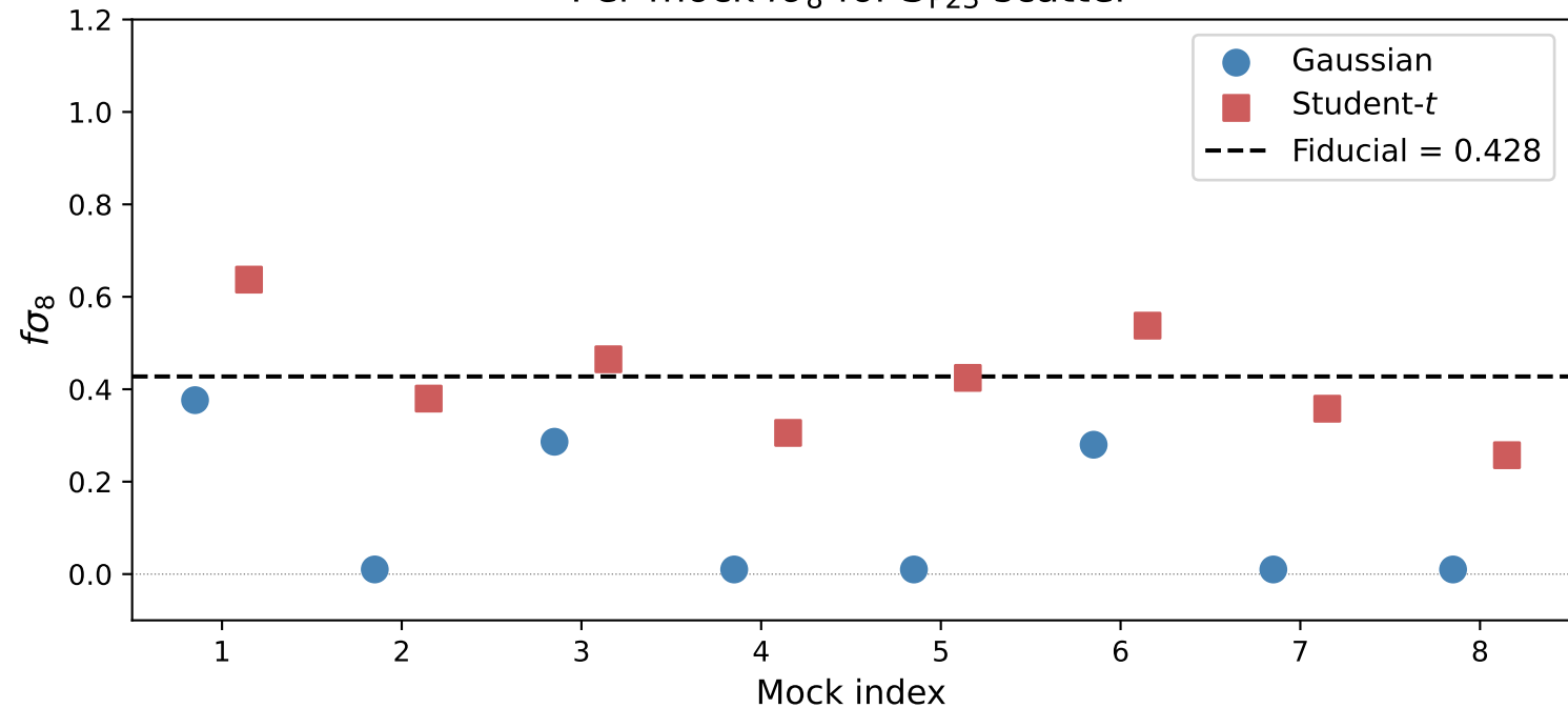
Per-mock f\sigma_8 for S_{P23} scatter
