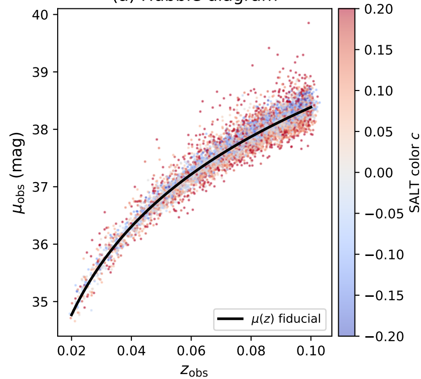
(a) Hubble diagram
