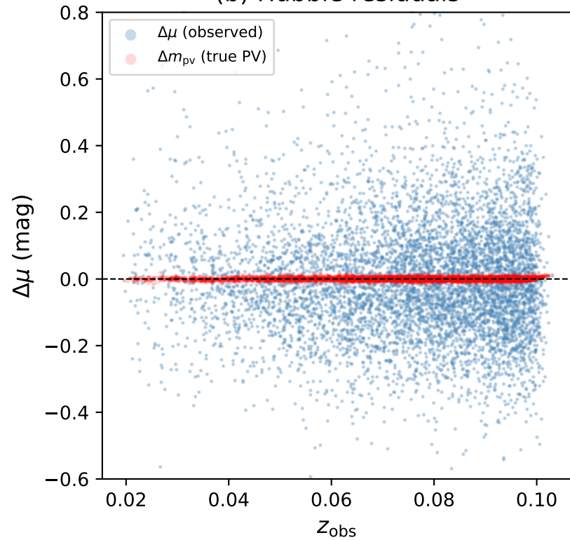
(b) Hubble residuals
