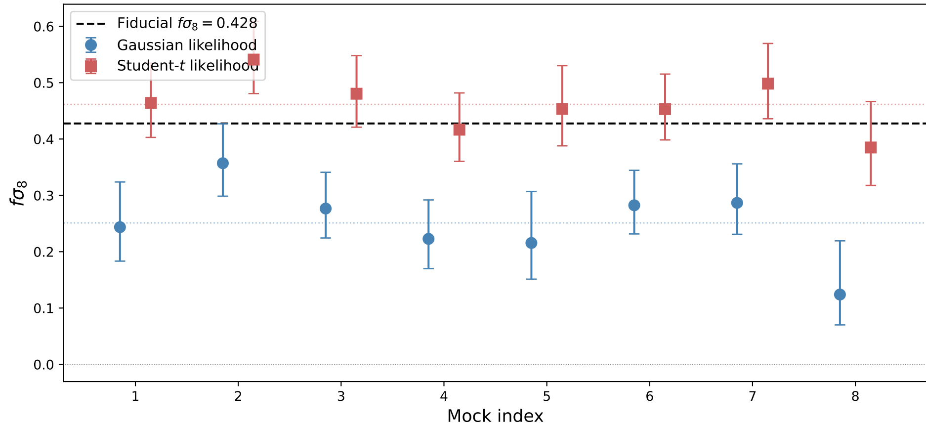
f\sigma_8 recovery: 6600 SNe \times 8 Uchuu mocks with S_{P23}
