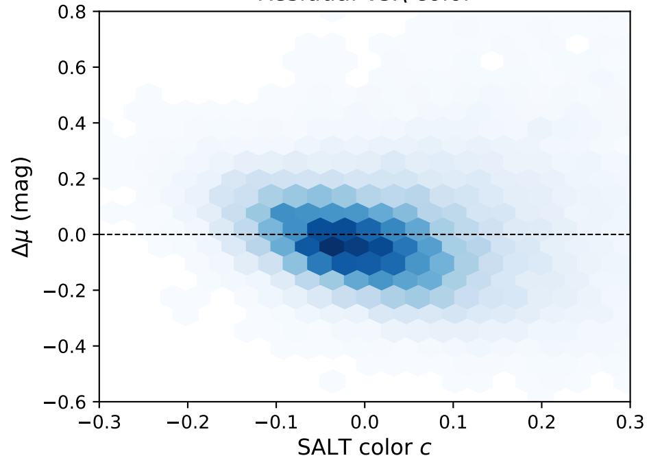
Residual vs. \ color
