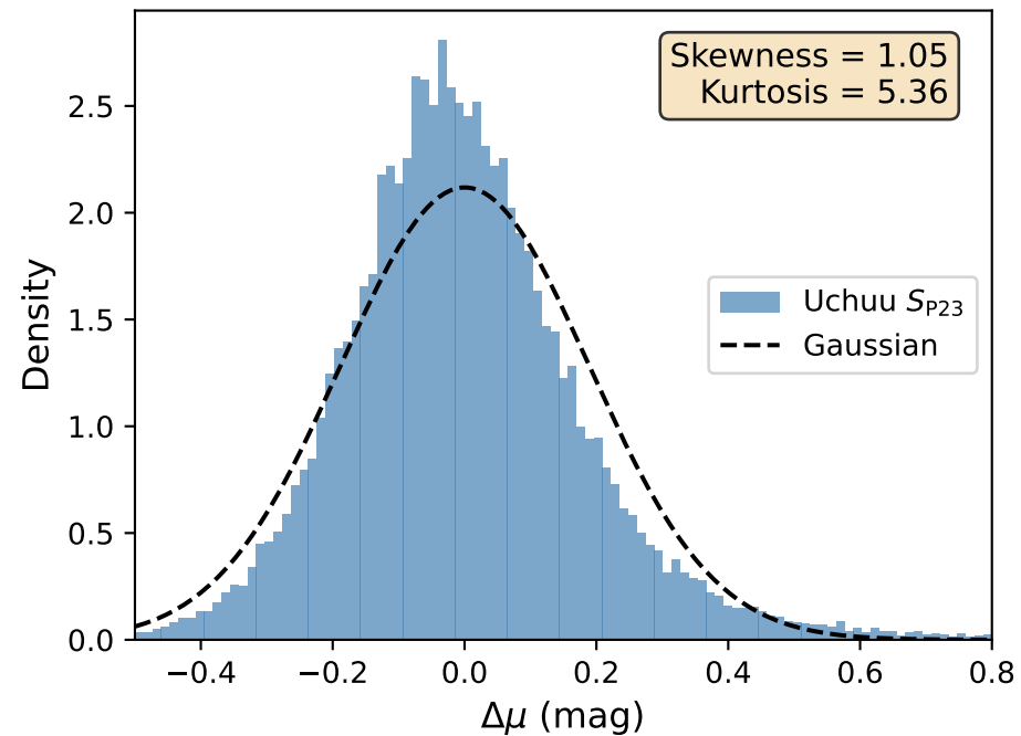
Hubble residuals (Uchuu + P23)
