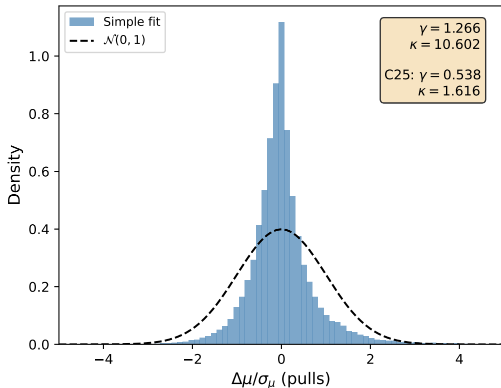
Pulls of Hubble residuals ( S_{P23} )
