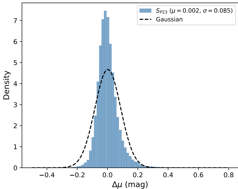
Hubble diagram residuals ( S_{P23} , SNANA)
