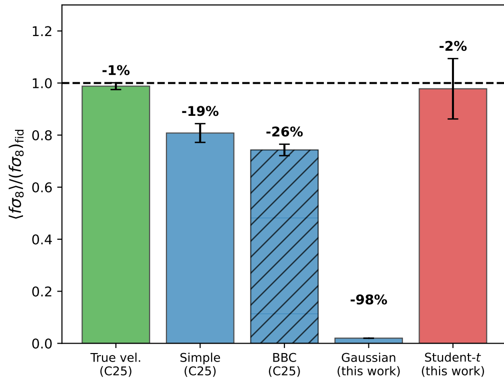
f\sigma_8 recovery for S_{P23} (cf. C25 Fig. 8)
