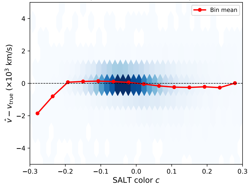
Velocity bias vs color (cf. C25 Fig. 7)
