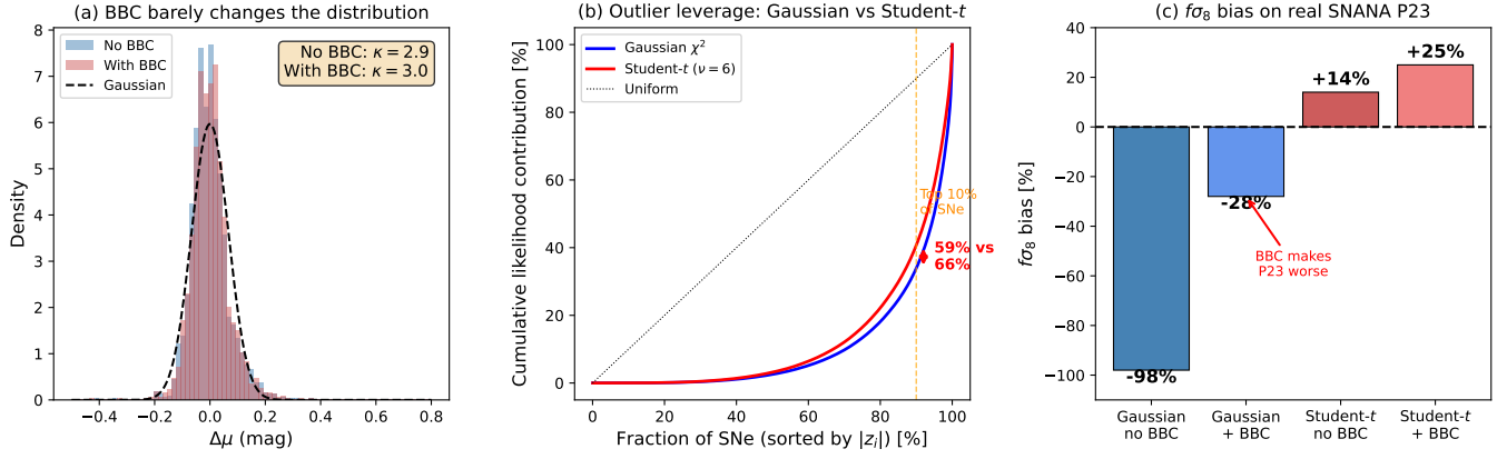
Figure 7. (a) BBC barely changes the Hubble residual distribution: kurtosis is \sim 3 with or without BBC. (b) Cumulative likelihood contribution sorted by residual size. In the Gaussian (blue), the top 10% of outlier SNe contribute 66% of \chi^2 . The Student- t (red) reduces this to 59%, breaking the outlier dominance. (c) f\sigma_8 bias on real SNANA P23 data (2125 SNe): the Student- t without BBC (+14%) outperforms Gaussian + BBC (−28%). BBC worsens both likelihoods.
