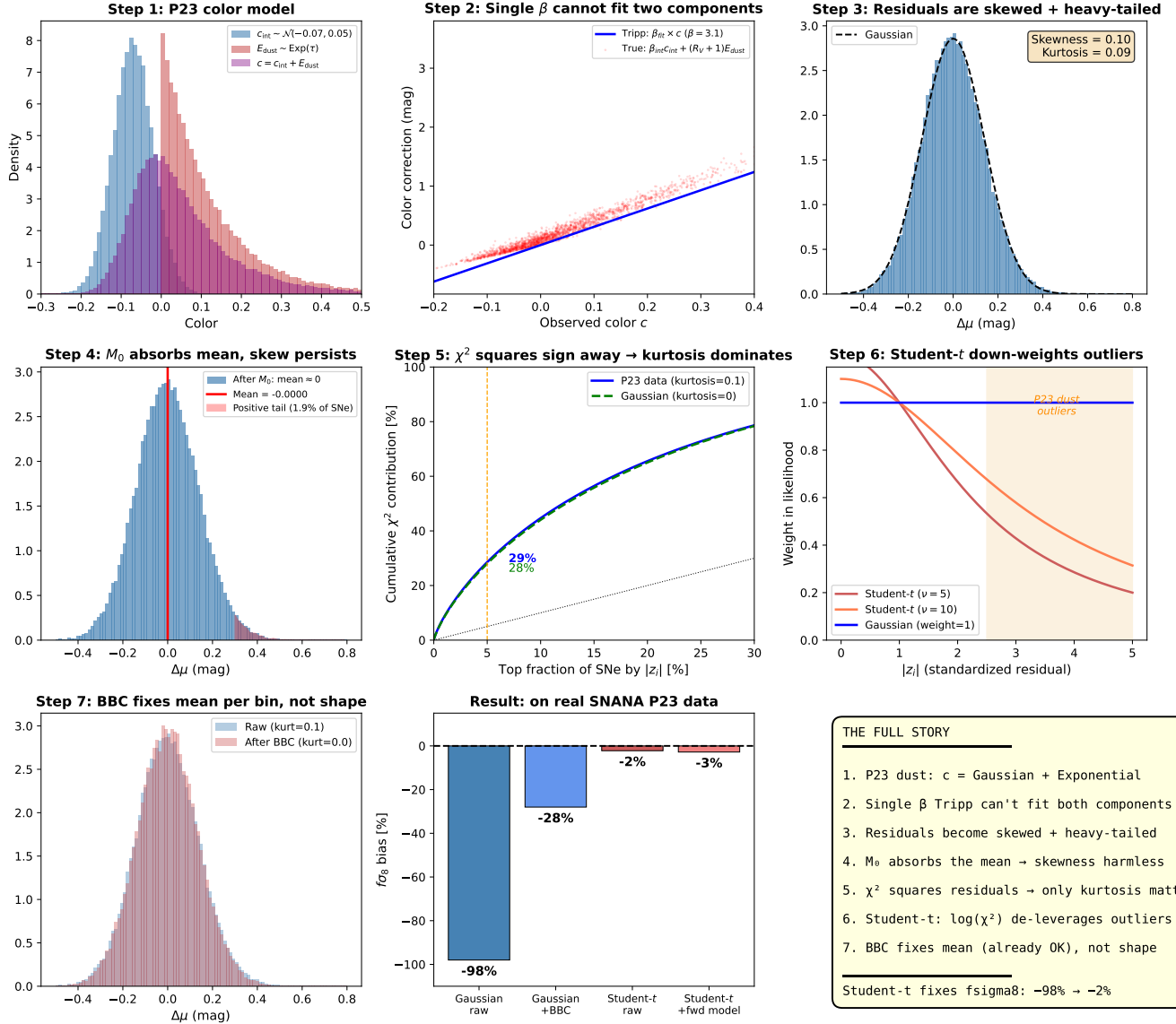
Figure 6. The complete causal chain from P23 dust to f\sigma_8 bias. Step 1: P23 color = Gaussian + Exponential. Step 2: Single Tripp \beta cannot fit two components. Step 3: Residuals become skewed and heavy-tailed. Step 4: M_0 absorbs the mean; skewness is harmless. Step 5: \chi^2 squares residuals, so only kurtosis biases f\sigma_8 . Step 6: Student- t down-weights outliers. Step 7: BBC fixes the mean (already OK), not the shape. Bottom middle: bias on real SNANA P23 data.
