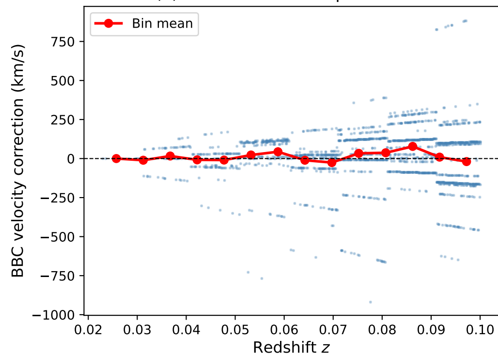
(a) BBC correction depends on z
