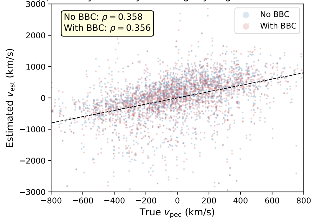
(c) Velocity recovery: BBC slightly degrades correlation
