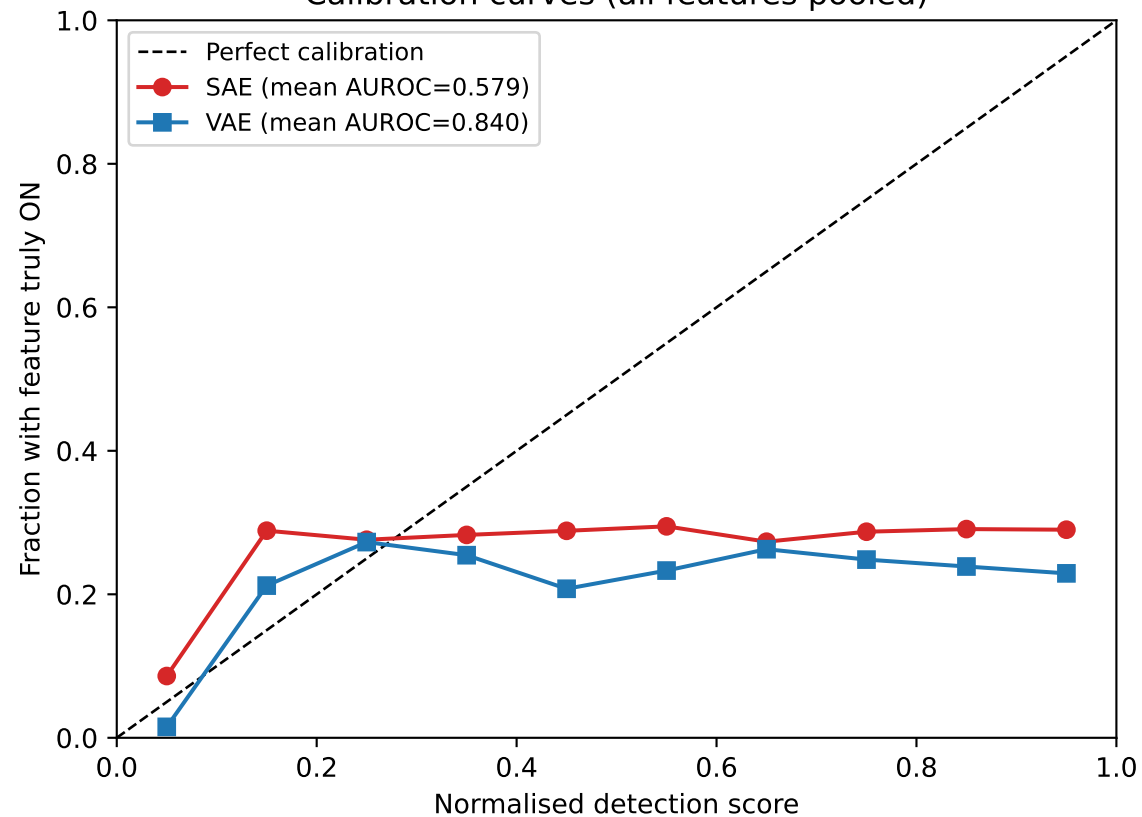
Calibration curves (all features pooled)
