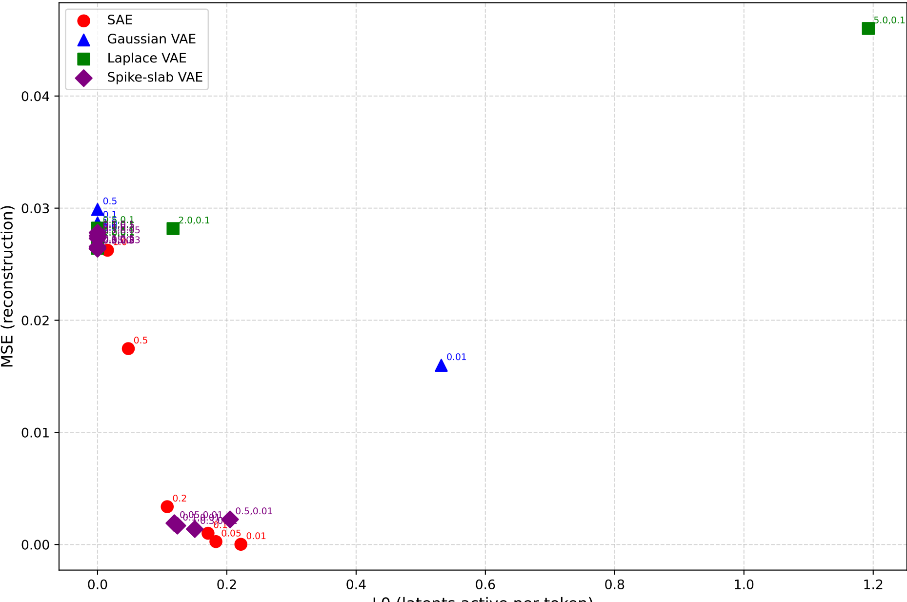
Pareto Frontier: MAP vs VI under different priors (Toy Superposition)
