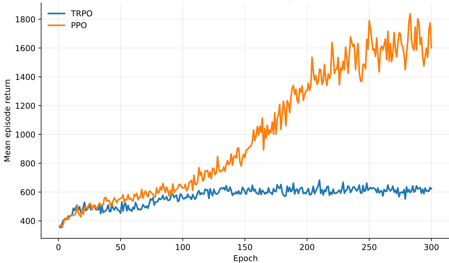
ALE/BeamRider-v5: training curves
