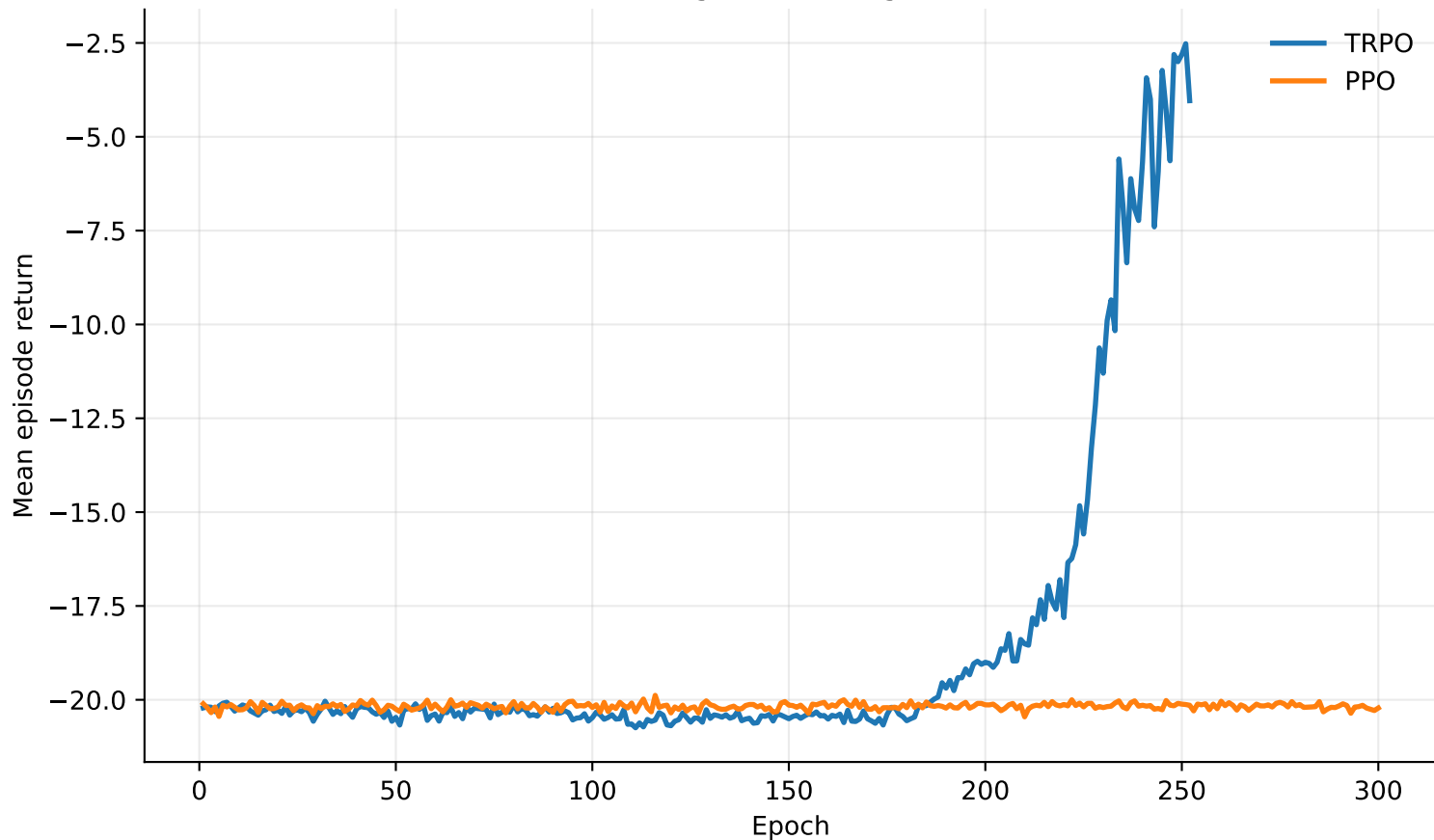
ALE/Pong-v5: training curves
