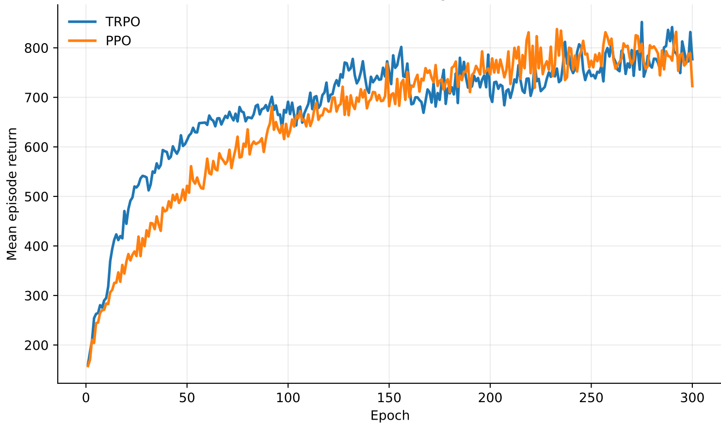
ALE/Qbert-v5: training curves
