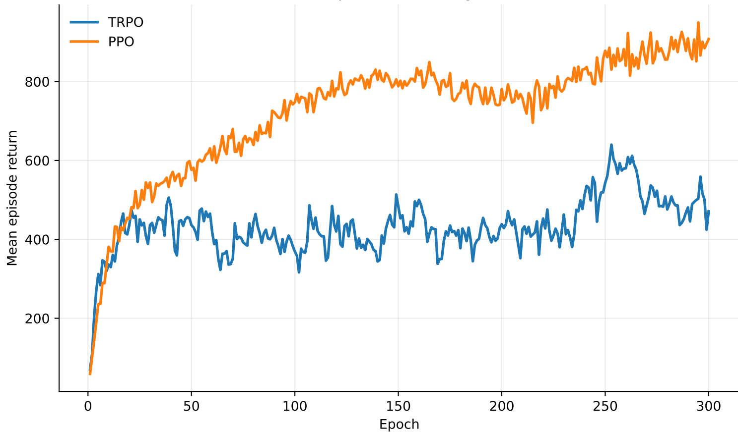
ALE/Seaquest-v5: training curves
