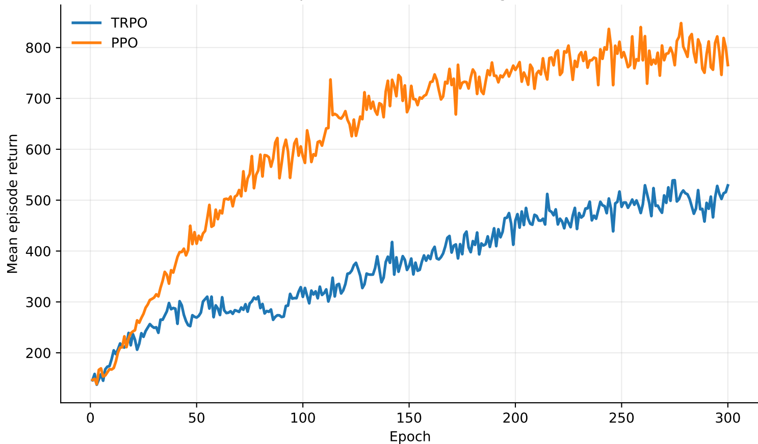
ALE/SpaceInvaders-v5: training curves
