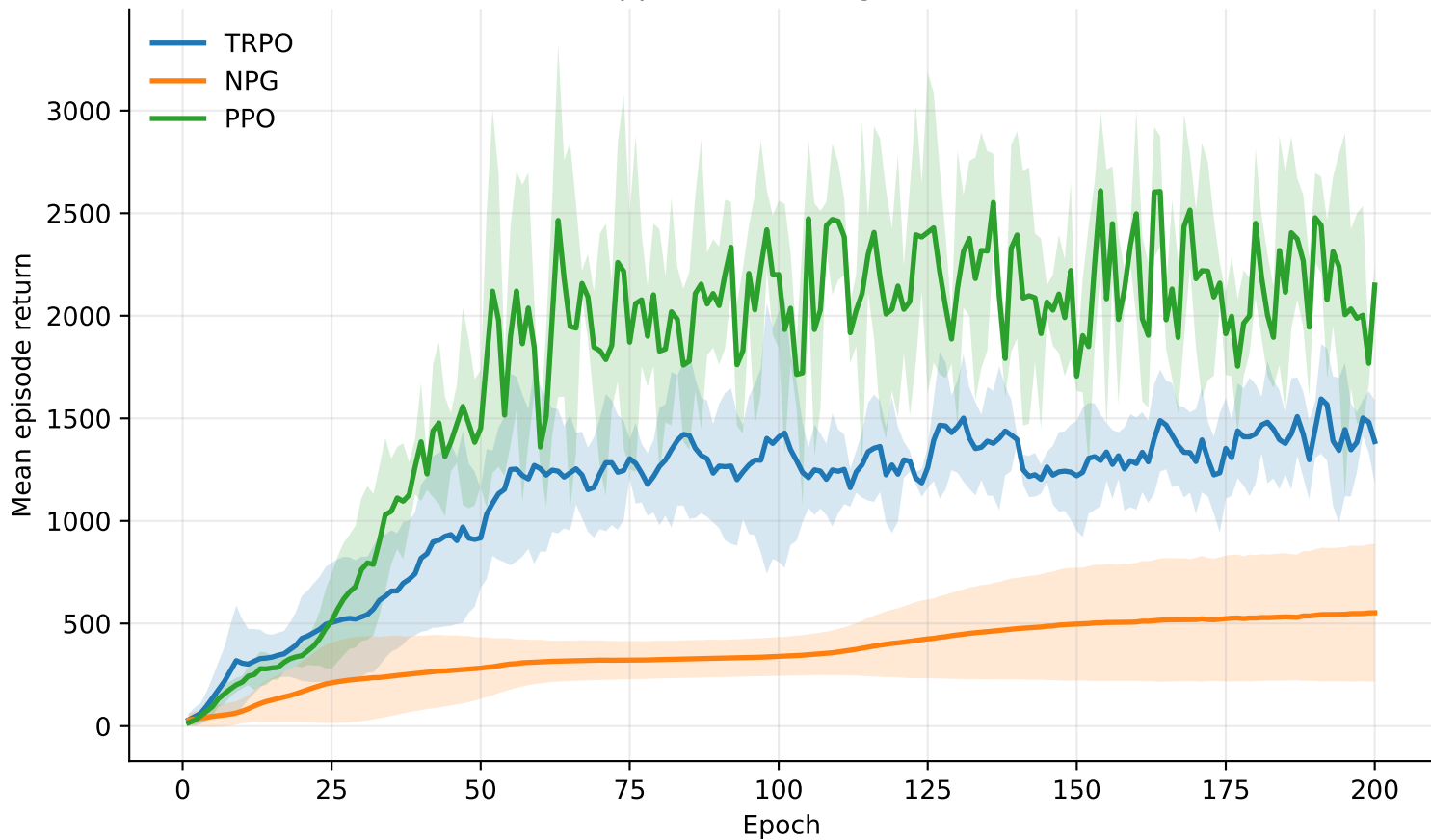
Hopper-v5: training curves
