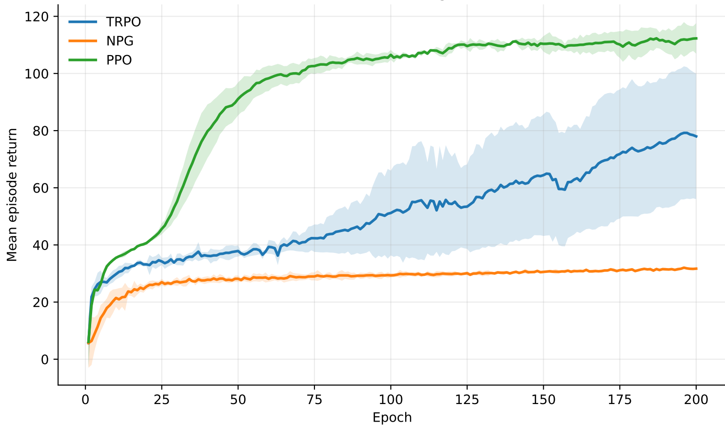
Swimmer-v5: training curves
