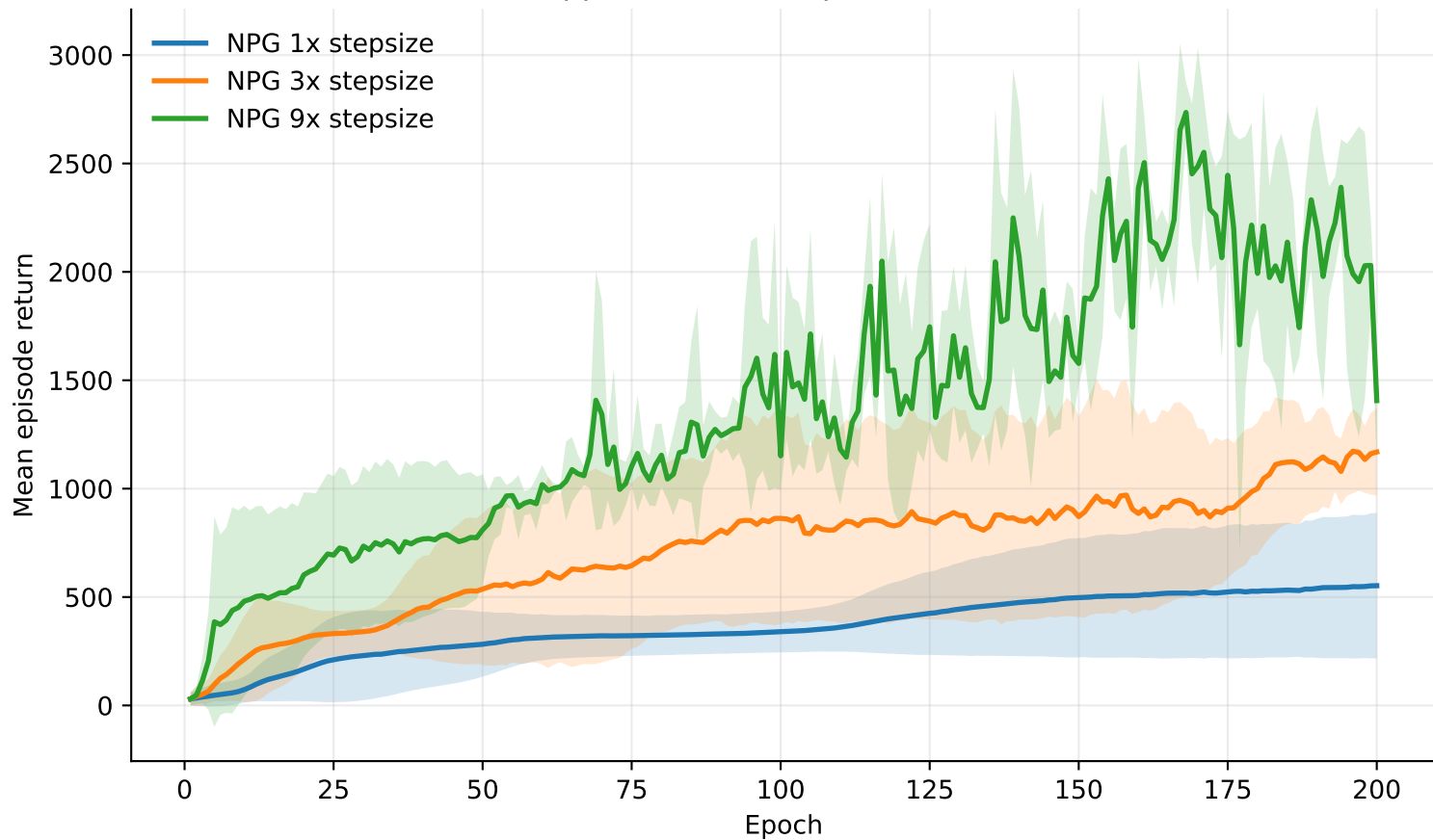
Hopper-v5: NPG step-size ablation
