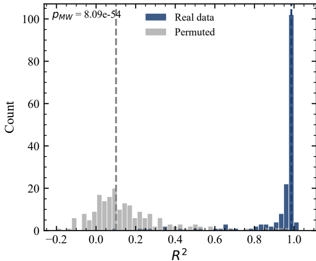
Y-Randomization Test
