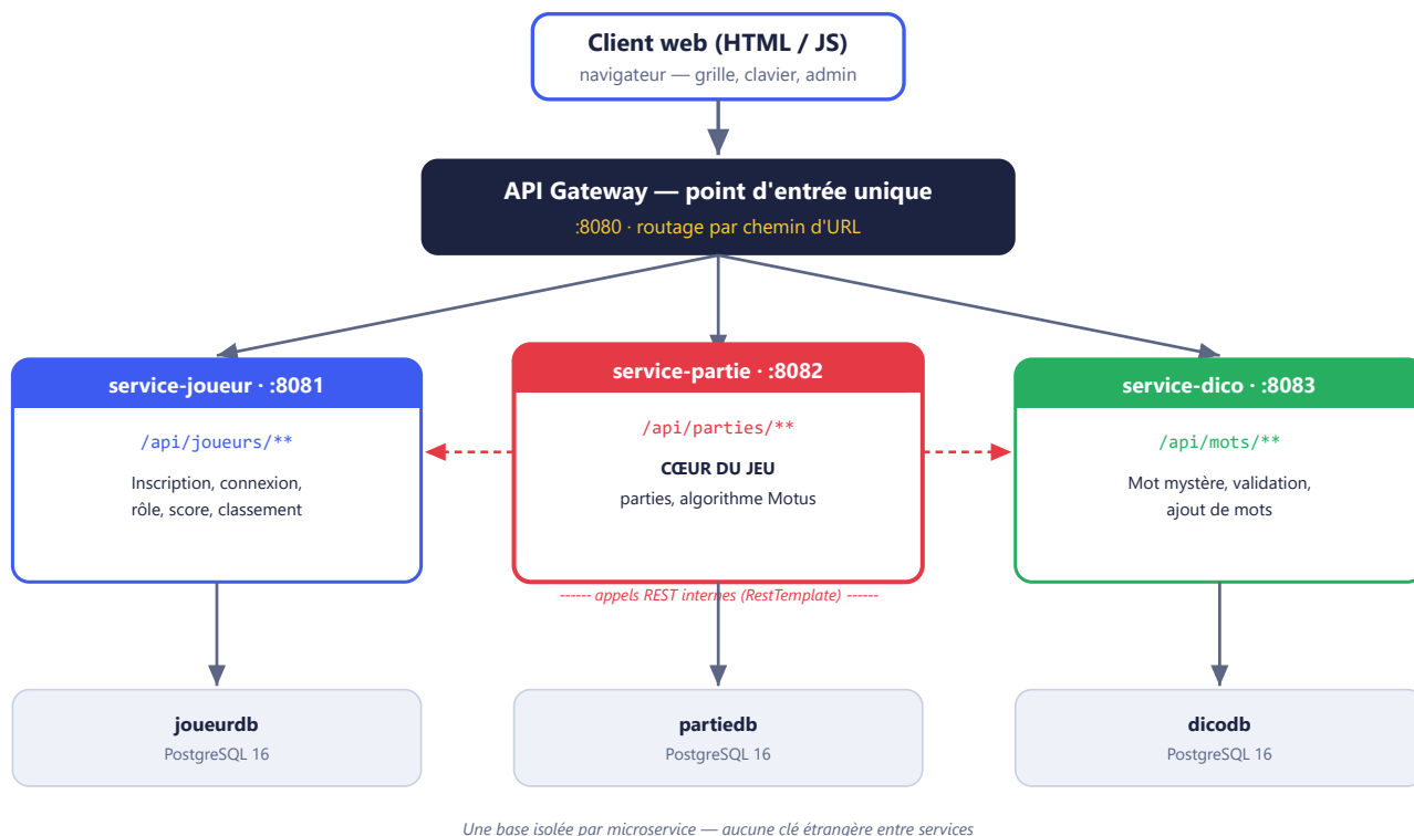
Figure 1 — Architecture microservices et flux de communication
