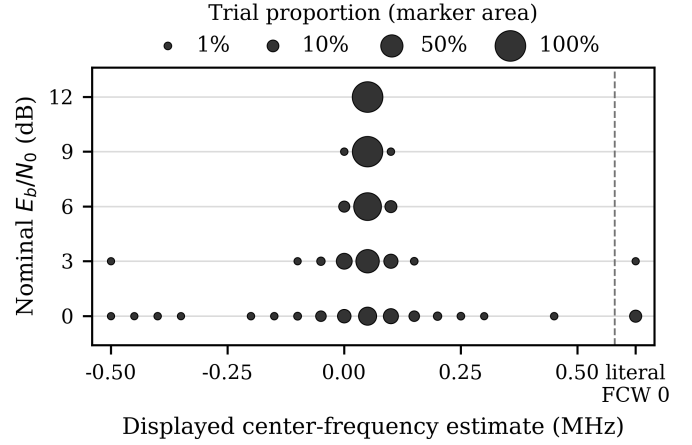
Fig. 10. Archived 300-record center-frequency rows for nominal E_b/N_0 values of 12, 9, 6, 3, and 0 dB. Marker area represents the trial proportion in each displayed bin. The final category preserves literal FCW zero records that do not map to the script's displayed frequency grid; it contains one record at 3 dB and 33 at 0 dB.
