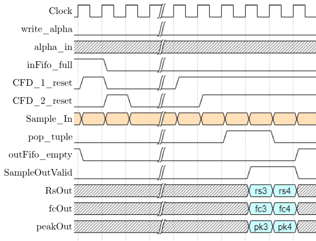
Fig. 12. Published output timing example. Later retained FIFO logic rejects a new write while full rather than discarding the oldest entry; source for the illustrated earlier behavior was not retained.
