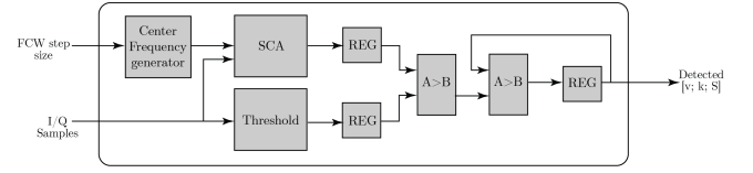
Fig. 8. Block diagram of the center-frequency detector module.
