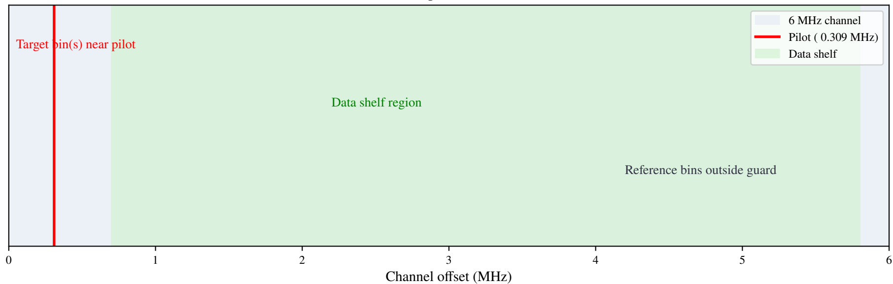
C. ATSC 1.0 pilot/data schematic
