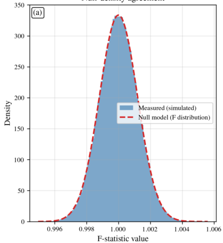
Null-density agreement
