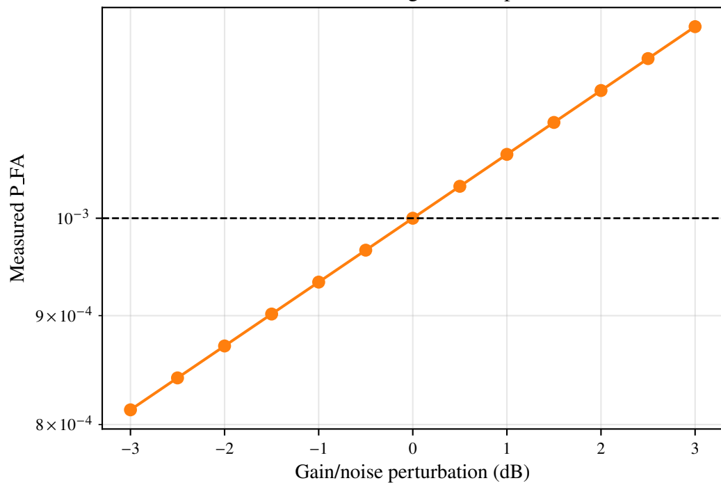
C. Measured P_FA vs gain/noise perturbation
