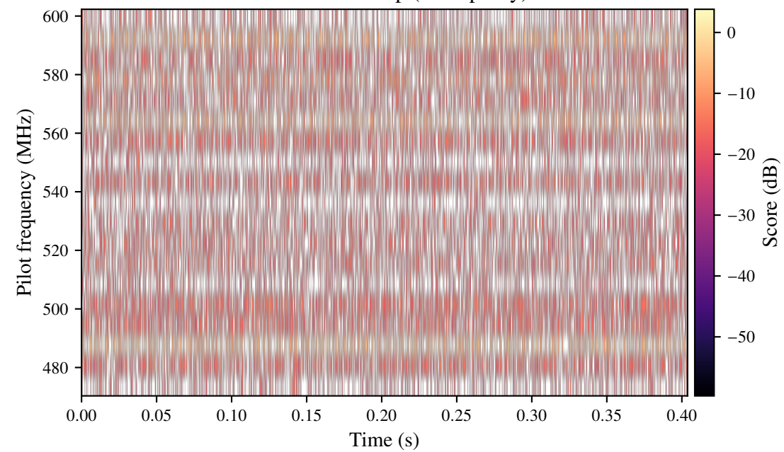
D. Expanded DTV mask
