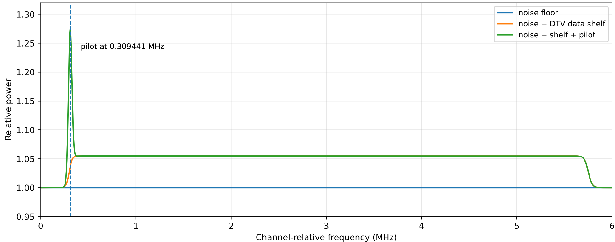
Synthetic ATSC channel components used in sensitivity studies
