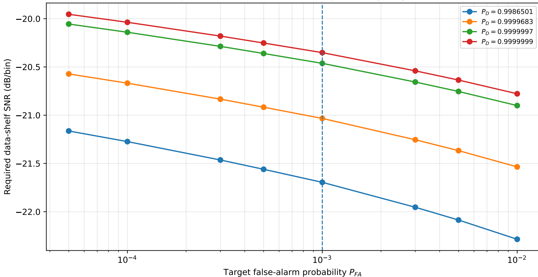
Required SNR for fixed detection-probability targets
