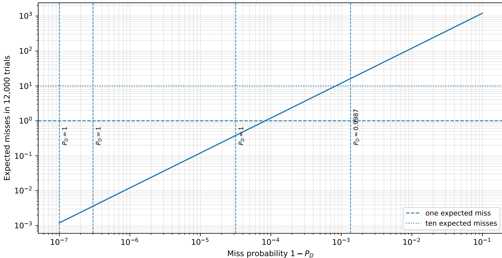
Finite-trial support for high detection-probability curves
