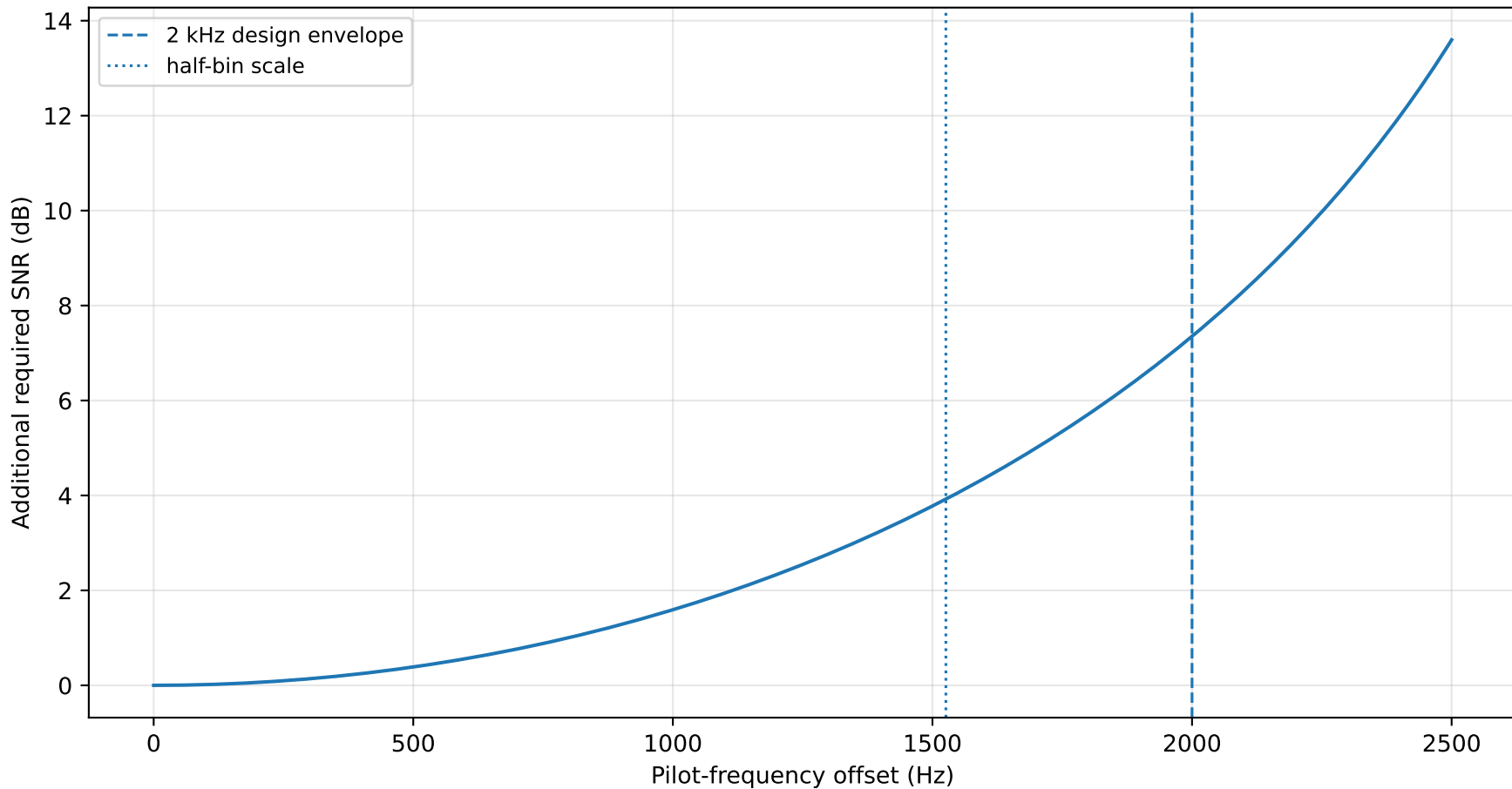
Frequency-offset penalty under a rectangular fine-bin response
