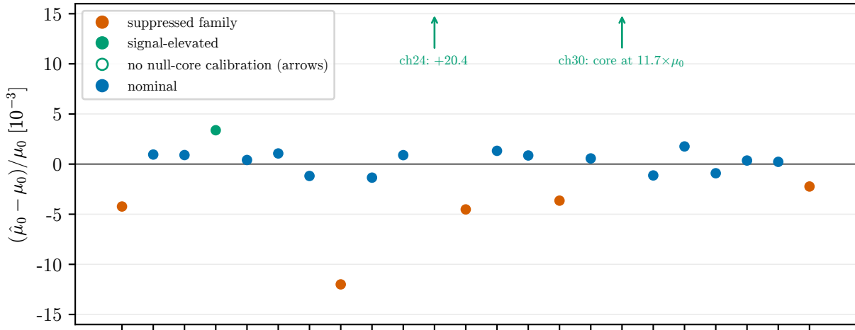
Measured vs analytic zero point (mode-anchored H0 core, full depth; per-event block-bootstrap errors)
