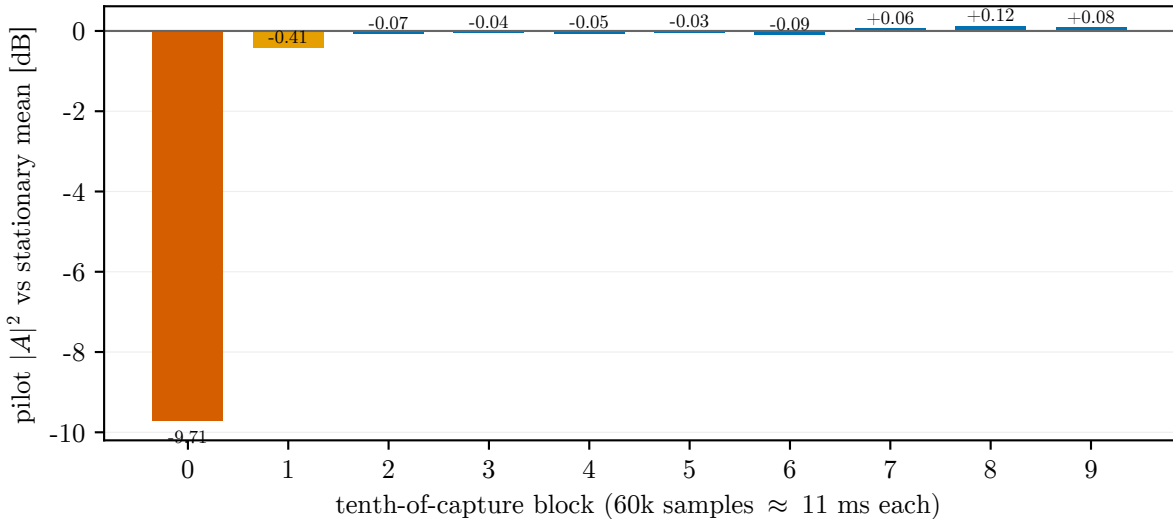
Golden-capture generator startup transient (T2 resolution): blocks 2--9 stationary
