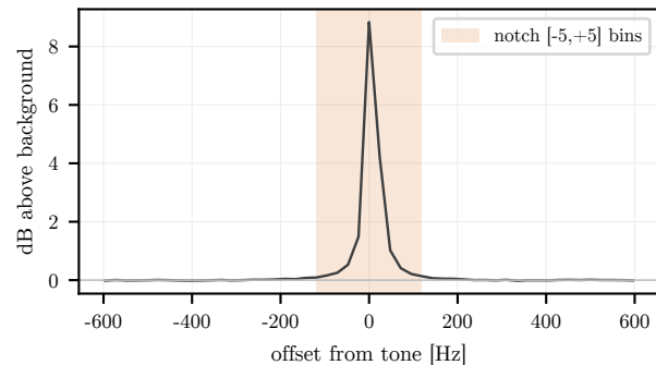
ch28: 8.8 dB at +130.200 kHz ( +SR/3 ) |f - +SR/3| = 7.9 Hz
