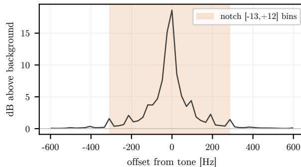
ch29: 18.6 dB at +156.260 kHz ( +2SR/5 ) |f - +2SR/5| = 9.5 Hz
