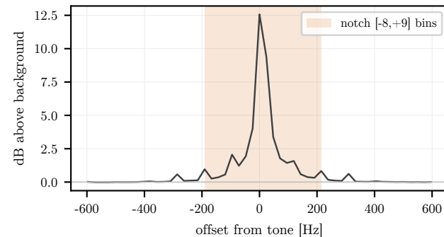
ch34: 12.6 dB at -156.260 kHz ( -2SR/5 ) |f - -2SR/5| = 9.5 Hz
