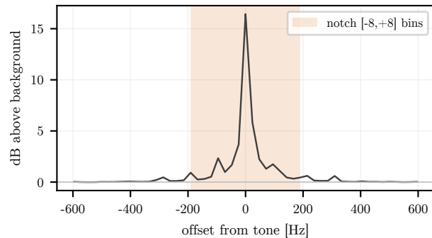
ch14: 16.4 dB at -78.130 kHz ( -SR/5 ) |f - -SR/5| = 4.8 Hz
