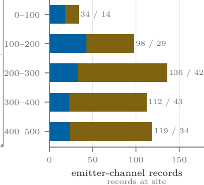
(c) records by range annulus
