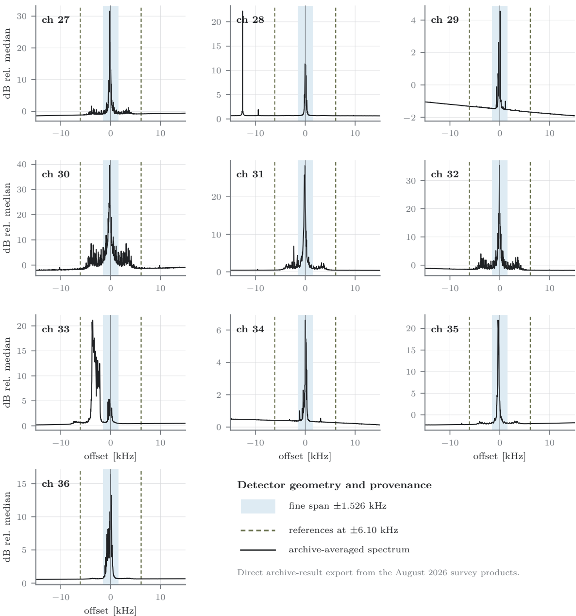
Archive-averaged spectrum around each pilot: main lobe, companions, and references
