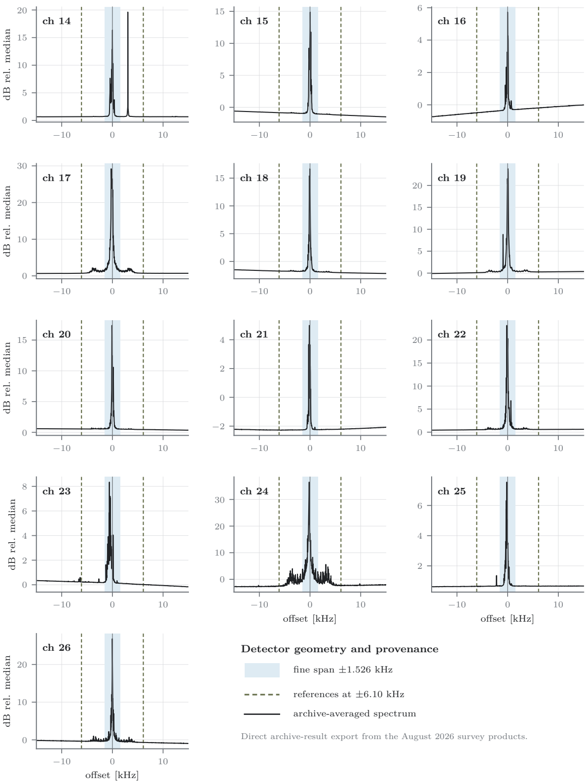
The lower band's spectral face: archive-averaged spectrum around each pilot, channels 14–26
