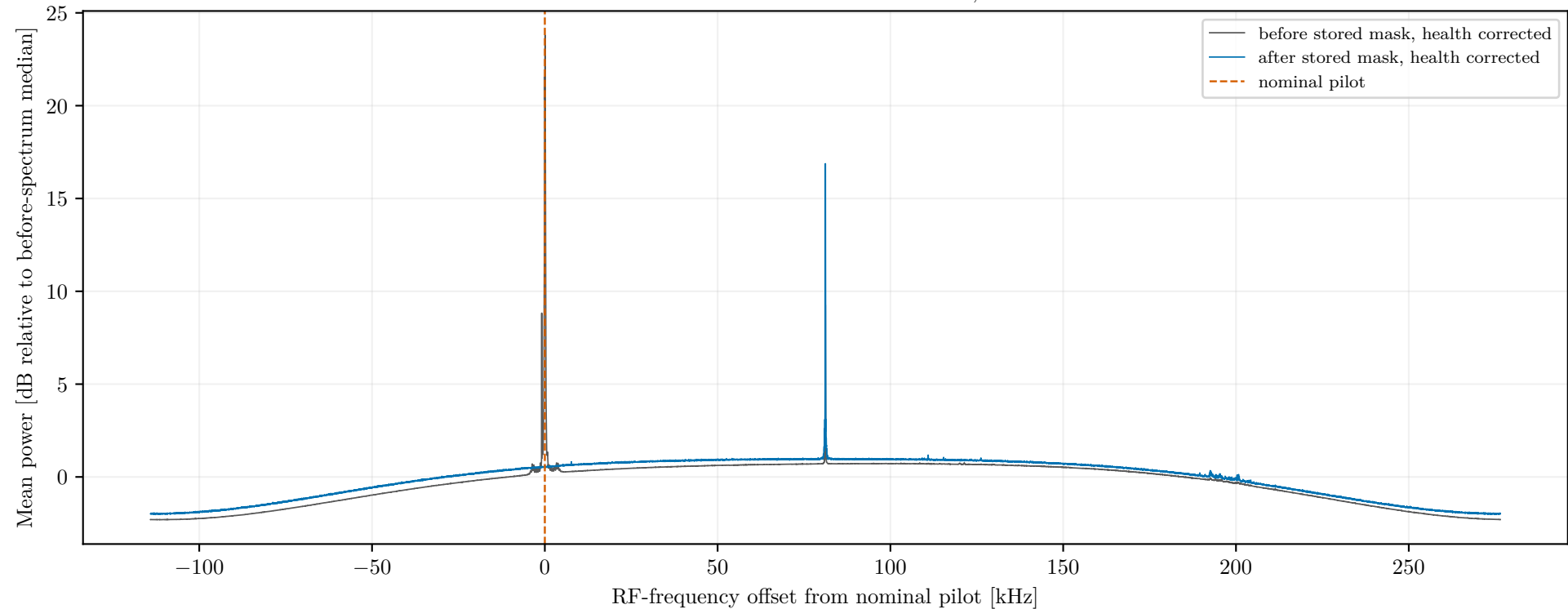
Channel 19 (frequency ID 767): relative time-averaged spectra exact v1 DC subtraction: 10 before, 10 after
