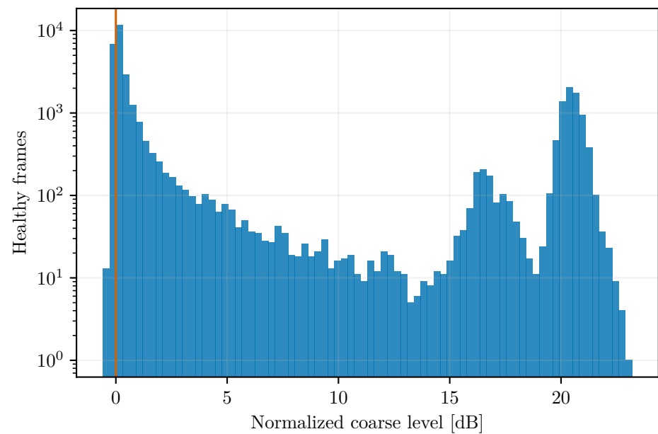
Channel 27 (frequency ID 644): health-filtered scalar distributions N=34,542; stored coarse mask rate 98.07%
