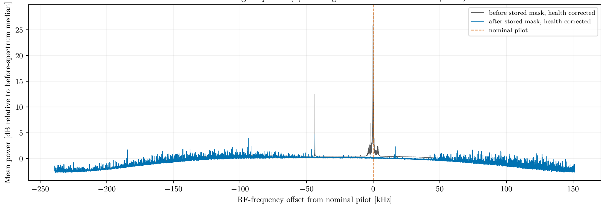
Relative time-averaged spectra (7/7 ceiling frames subtracted before/after)
