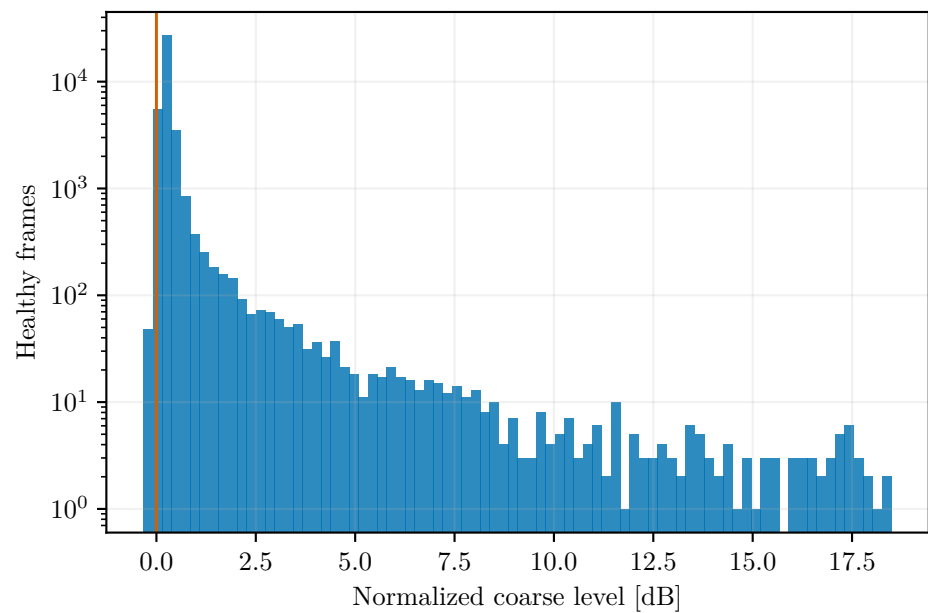
Channel 34 (frequency ID 537): health-filtered scalar distributions N=39,012; stored coarse mask rate 99.09%
