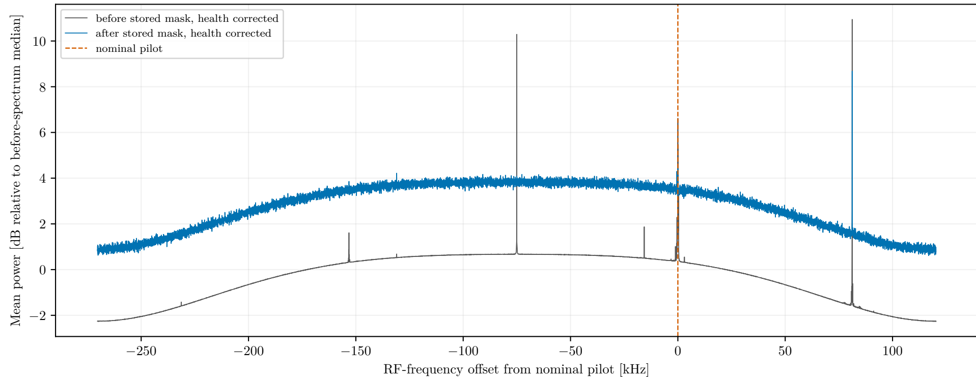
Channel 34 (frequency ID 537): relative time-averaged spectra exact v1 DC subtraction: 5 before, 0 after
