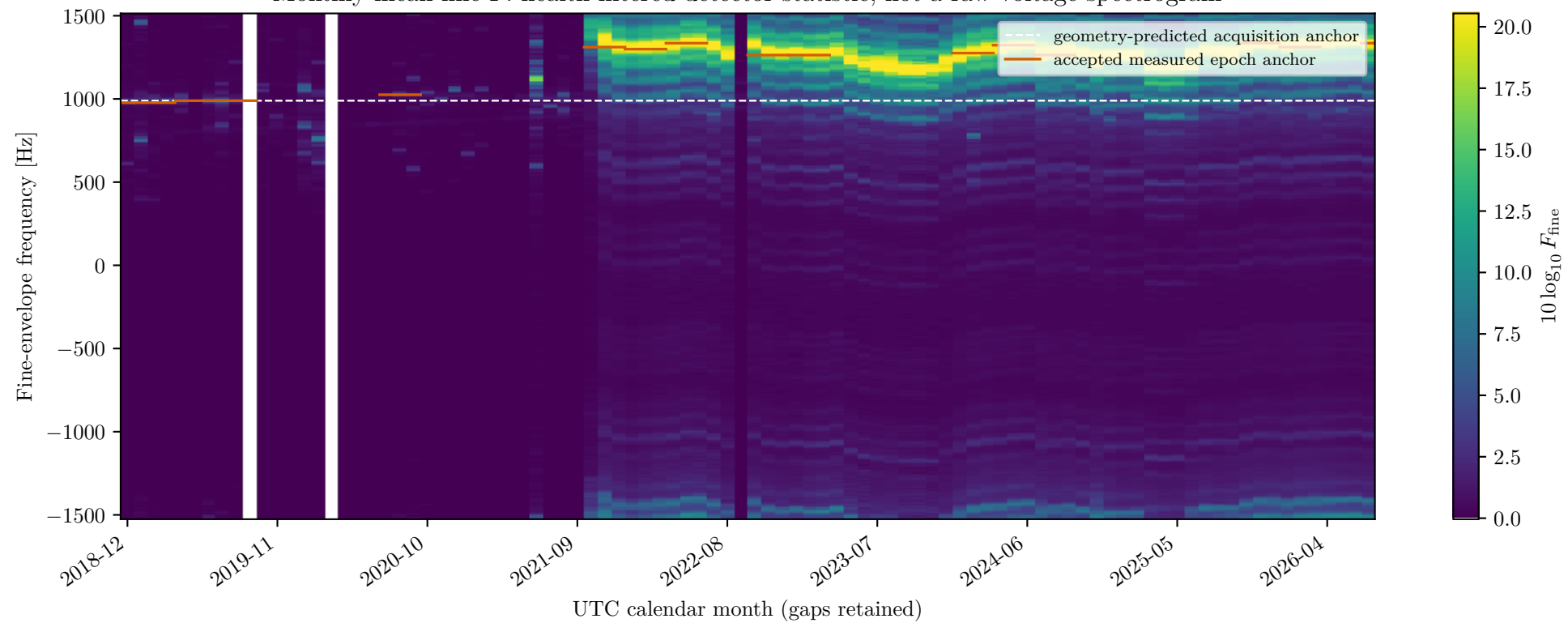
Monthly mean fine F: health-filtered detector statistic, not a raw-voltage spectrogram
