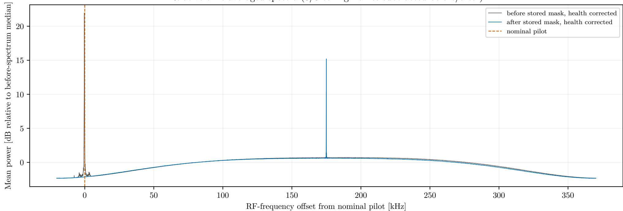
Relative time-averaged spectra (8/8 ceiling frames subtracted before/after)
