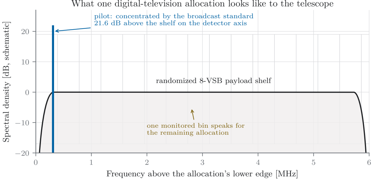
Figure 1.8: What one television allocation looks like to the telescope (schematic, drawn to the measured proportions). The 6 MHz shelf is the broadcast’s randomized data payload; in narrow time–frequency cells it can approach the null assumed by power- and variability-based flaggers. The pilot carries about 7% of the station’s power at a nominal standard-defined offset [2]: weak in total, but 21.6 dB above the shelf power integrated over the declared 3.052-kHz coarse analysis cell under the transmitter-ratio and flat-allocation convention used here. This is a finite-bandwidth power comparison, not a resolution-independent line PSD. CHIME’s 390.625 kHz channel raster is drawn behind; the detector monitors the bin containing the pilot as a proxy for the 15.36 bins spanned by the allocation. Chapters 3 and 4 derive the geometry and state the transfer assumptions.
