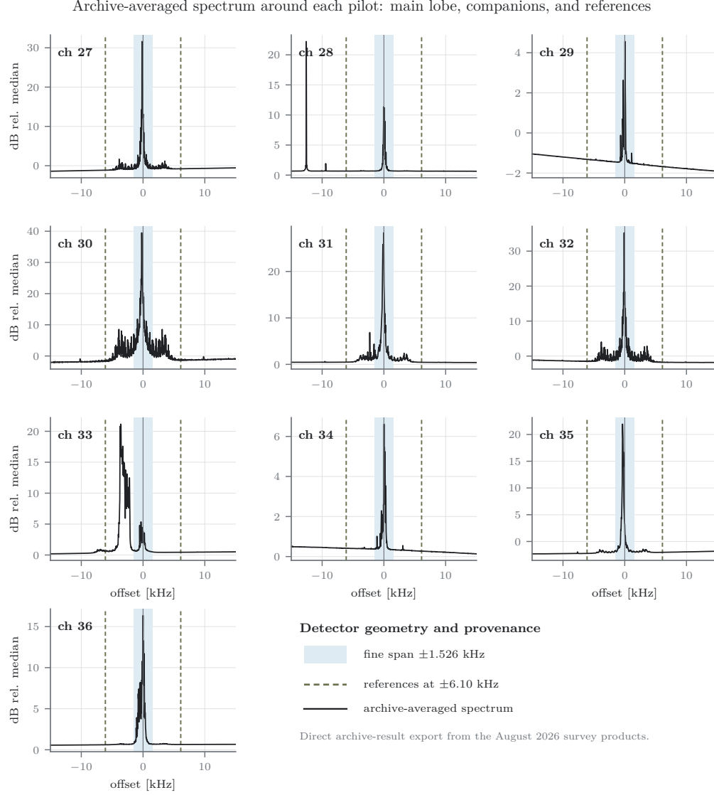
Figure 3.3: The transmitter population’s spectral face: archive-averaged spectrum within \pm 15 kHz of each pilot, from the survey products’ stored integrated spectra (dB relative to the channel median). Shaded: the K = 128 fine span ( \pm 1.526 kHz); dashed: the \pm 2 -bin reference placements ( \pm 6.1 kHz). Panels are centred on each channel’s synthesized (nominal) pilot in the transmitted-frequency sense, so a carrier’s displacement from zero is its measured off-nominal offset. On eight of the ten channels the dominant carrier is a single compact lobe inside the fine span, within 0.4 kHz of synthesis; on the crowded-field channels (30, 31, 32) it stands over the resolved sidelobe forest discussed in the text. Channel 33 is a documented exception: its globally dominant carrier sits at -3.6 kHz, in the skipped guard between the fine span and the lower reference, with companion structure near -2.6 kHz. It is outside the configured capture span even though a weaker nominal/in-span lobe remains available to the detector. Channel 28’s strongest feature in the displayed \pm 15 -kHz panel lies 12.6 kHz below synthesis, likewise far outside the capture geometry; it is not an “in-window” feature, while the nominal pilot stands at 11 dB. The references sit in clean territory on every channel — the placement validation of Section 4.1 made visually. The thirteen lower-band channels appear in Figure 9.7.
