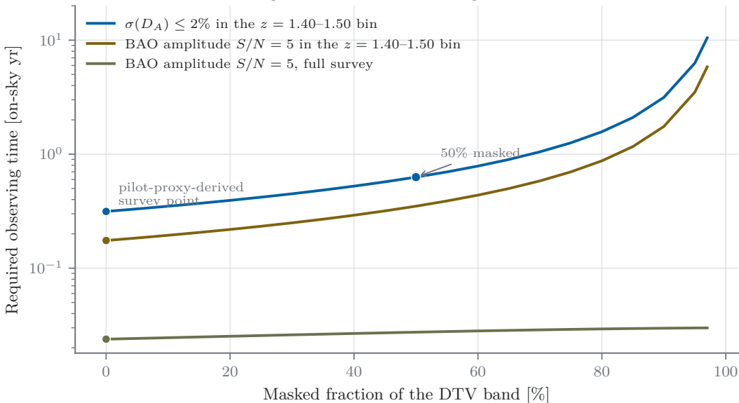
Noise tolerance: observing time to reach BAO targets versus uniform DTV masking
