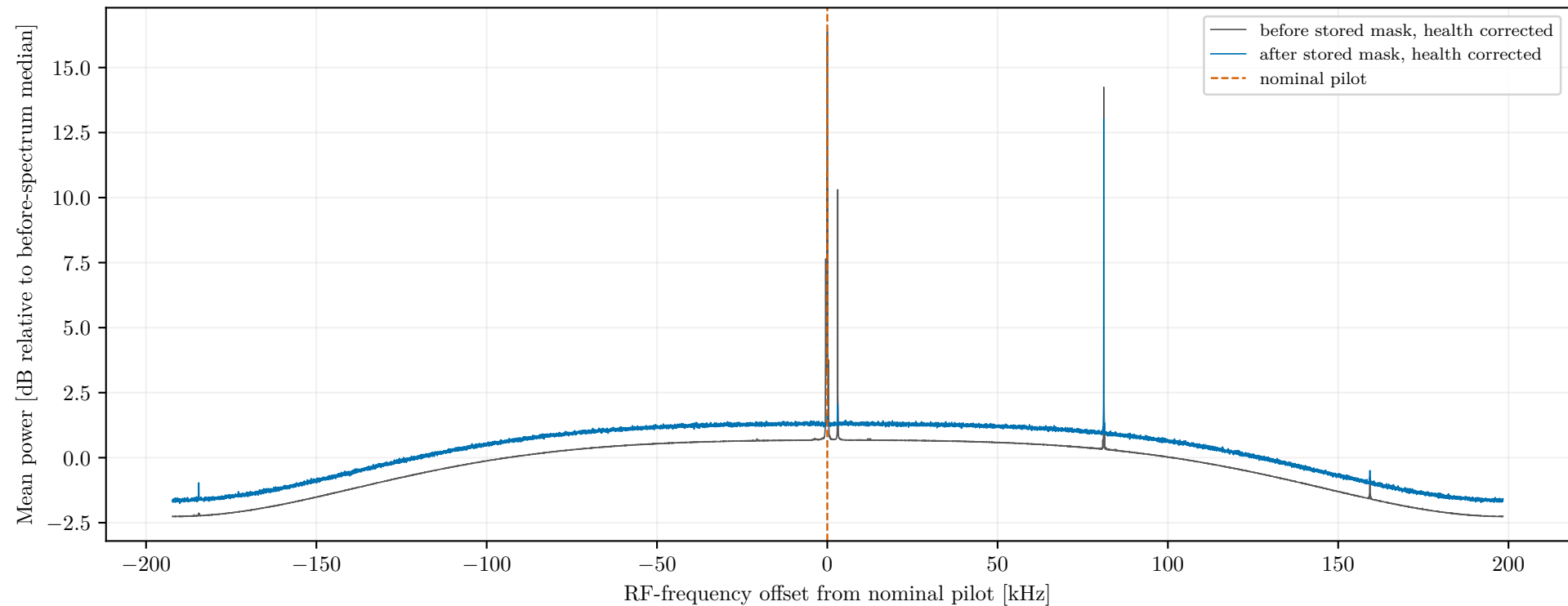
Channel 14 (frequency ID 844): relative time-averaged spectra exact v1 DC subtraction: 7 before, 0 after
