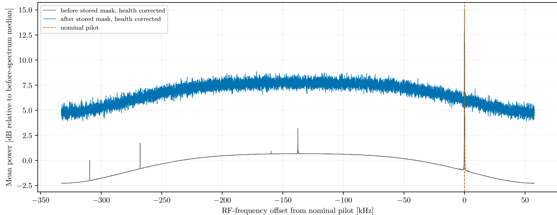
Channel 15 (frequency ID 829): relative time-averaged spectra exact v1 DC subtraction: 7 before, 7 after
