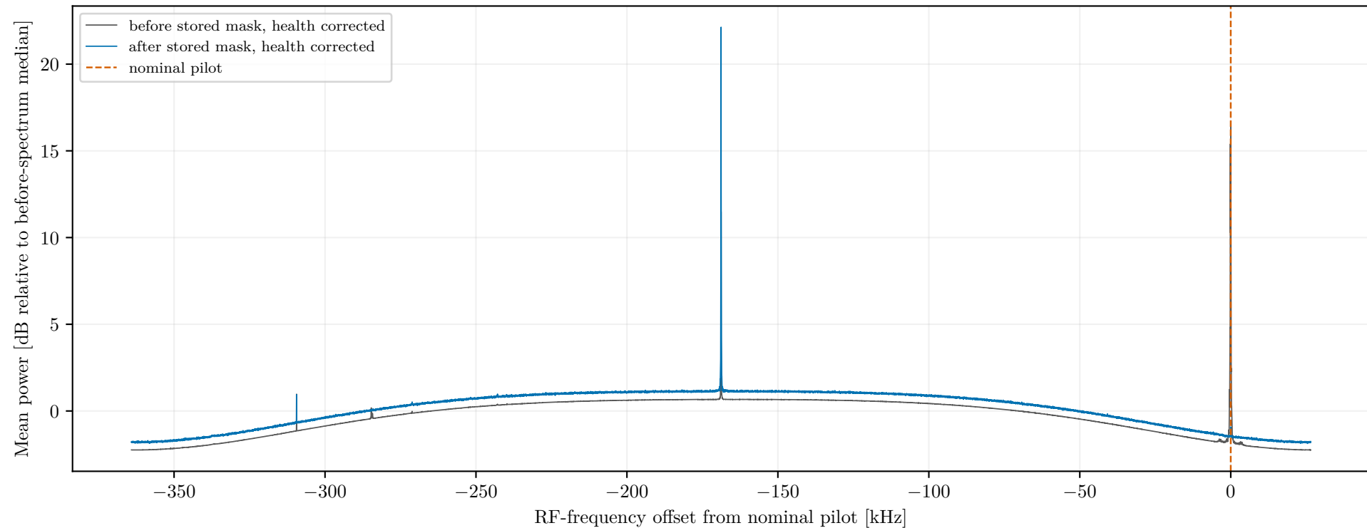
Channel 18 (frequency ID 783): relative time-averaged spectra exact v1 DC subtraction: 6 before, 6 after
