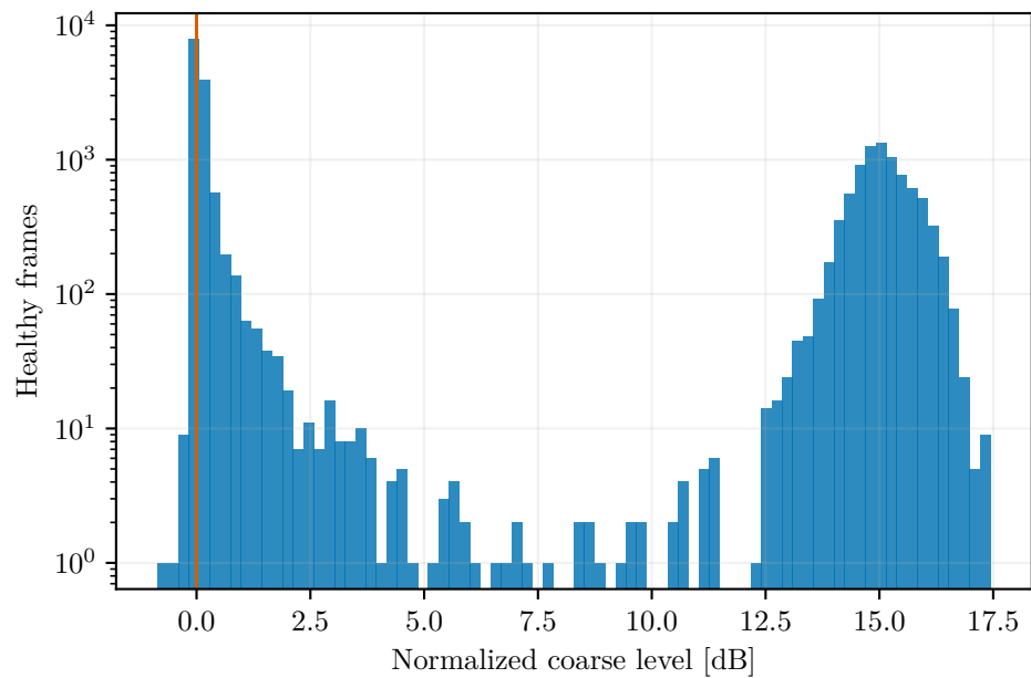
Channel 19 (frequency ID 767): health-filtered scalar distributions N=21,362; stored coarse mask rate 91.80%
