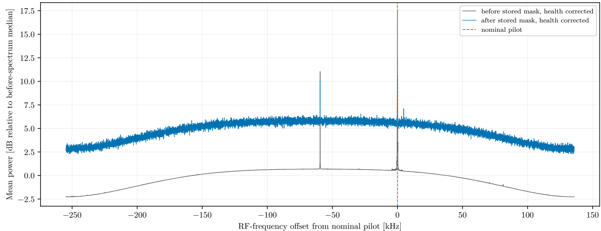
Channel 20 (frequency ID 752): relative time-averaged spectra exact v1 DC subtraction: 9 before, 0 after
