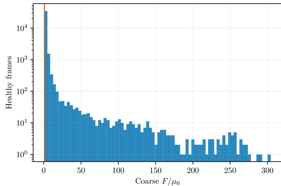
Channel 22 (frequency ID 721): health-filtered scalar distributions N=37,959; stored coarse mask rate 100.00%
