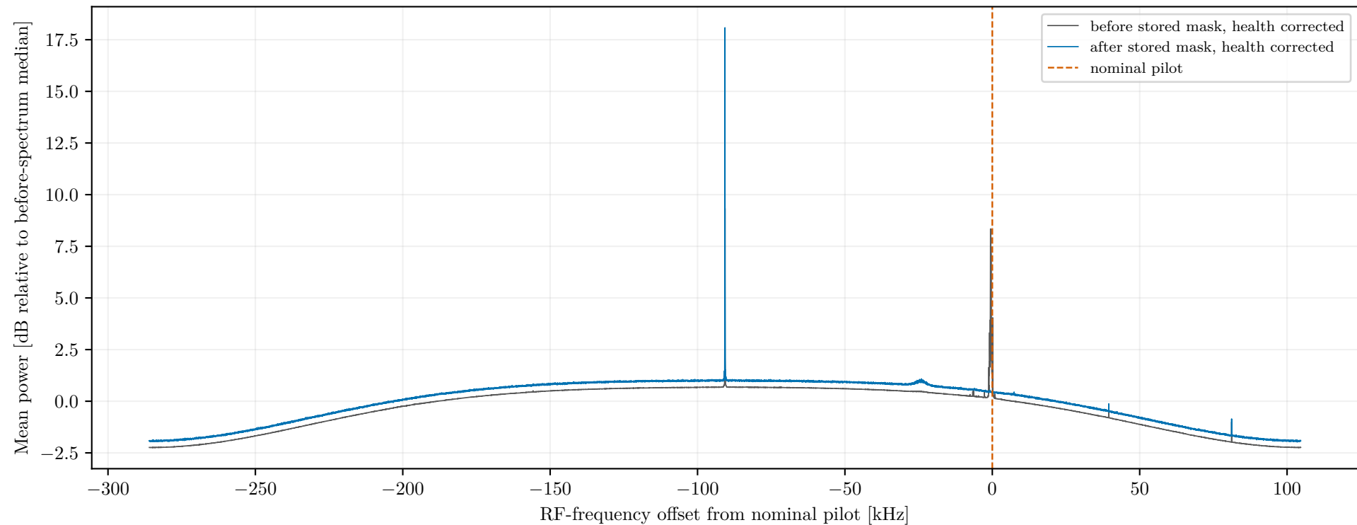
Channel 23 (frequency ID 706): relative time-averaged spectra exact v1 DC subtraction: 7 before, 7 after
