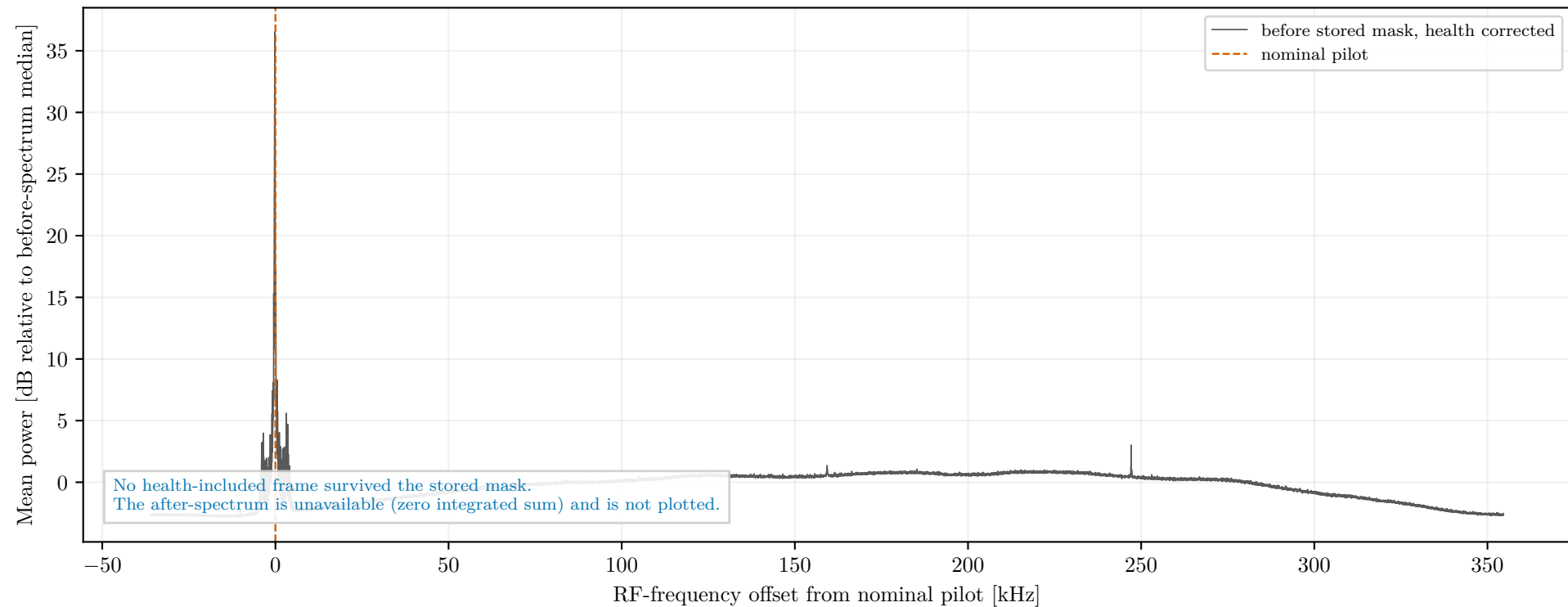
Channel 24 (frequency ID 690): relative time-averaged spectra exact v1 DC subtraction: 2 before, 2 after
